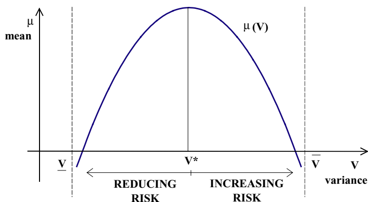
Figure 1. Mean variance schedule, \mu(V) , for earnings.
