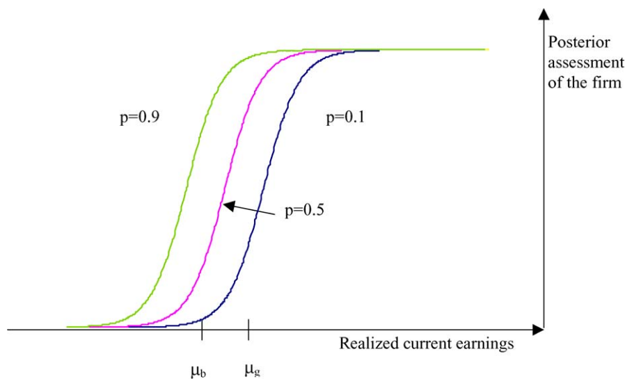
Figure 2. Posterior probability that a firm is good, as a function of realized current earnings, for various values of p , the prior probability that a firm is good.
