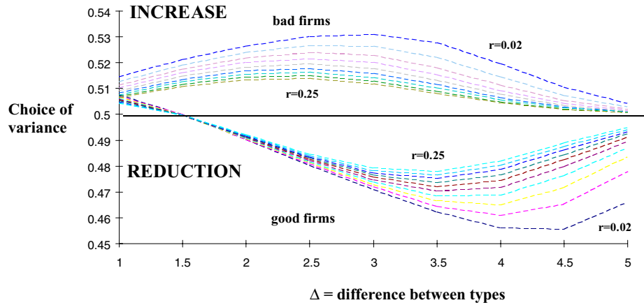
Figure 5. Risk reduction and increase as a function of the difference between types ( \Delta ) and the discount rate r ( p is fixed at 0.1).
