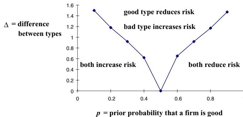
Figure 4. Threshold value of \Delta (the difference between types) as a function of p (the prior probability that a firm is good).
