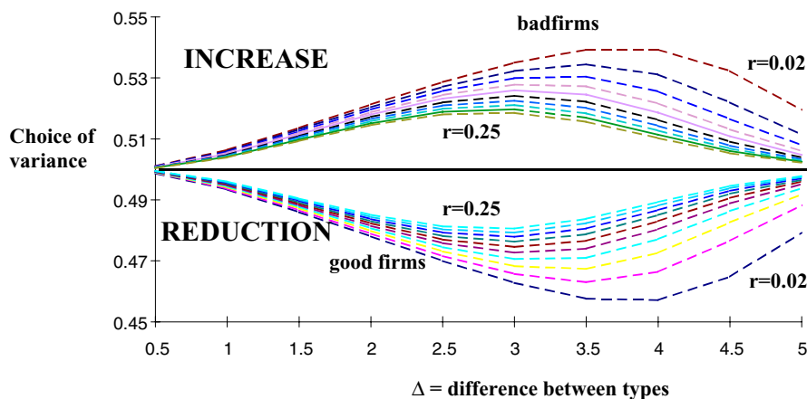
Figure 3. Risk reduction and increase as a function of the difference between types ( \Delta ) and the discount rate r ( p is fixed at 0.5).
